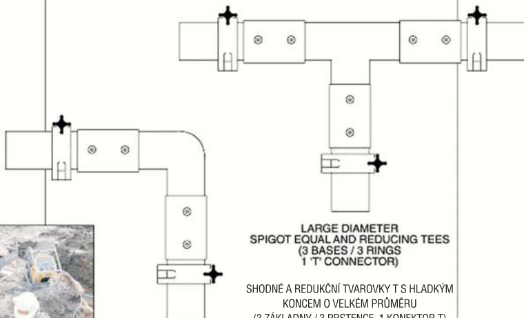
ELECTROFUSION OF 90° SPIGOT ELBOWS (2 BASES 1 T' CONNECTOR)
